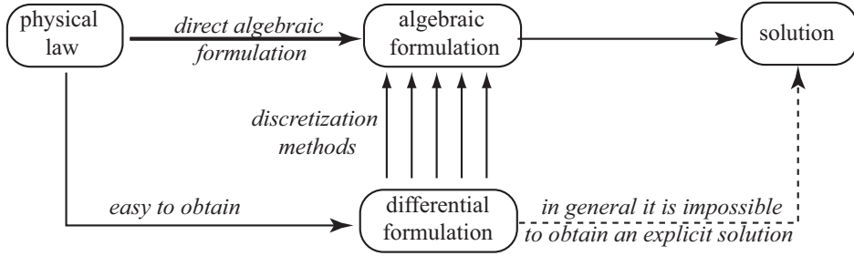
Figure 2. The direct algebraic formulation: the Cell Method .
