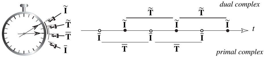
Figure 3. A primal cell complex in time and its dual.
