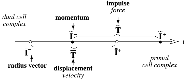
Figure 6. The association of variables of particle dynamics with time elements. Global variables are in bold.
