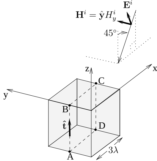
Figure 4.1: 3\lambda \times 3\lambda \times 3\lambda PEC cube illuminated by a plane wave with \hat{y} -polarized magnetic field. The direction of incidence forms a 45^\circ angle with the \hat{z} - axis. The points A, B, C, and D define a closed curve denoted ABCDA.
