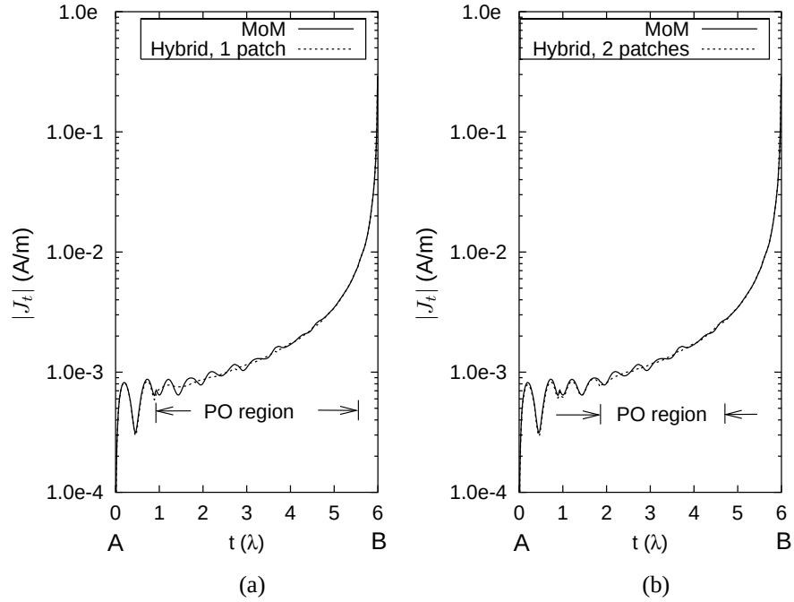
Figure 6.5: Surface current density along the curve AB obtained with MoM and hybrid PO-MoM. The component along AB is shown. In (a), the MoM region is one patch wide. In (b), the MoM region is two patches wide.
