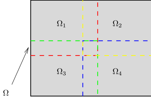
Figure 4.4: Domain \Omega divided into four overlapping subdomains. \Omega_1 is bounded by the red curve, \Omega_2 by the yellow curve, \Omega_3 by the green curve, and \Omega_4 by the blue curve.
