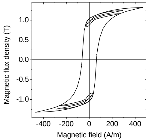
Fig. 8. CASE2: computed hysteresis loop in point C6.
