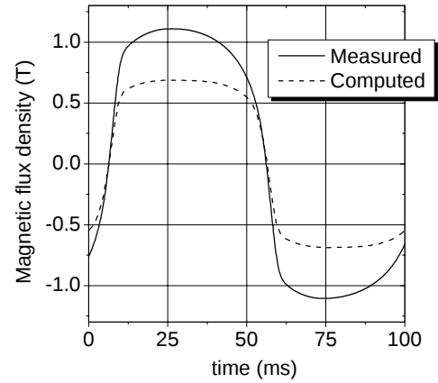
Fig. 4. CASE1: computed and measured waveform of magnetic flux density in the left limb (coil C5).
