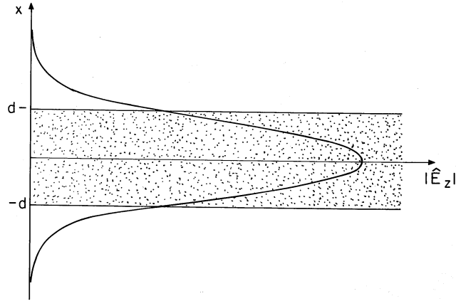
Fig. 13.5.4 Distribution of transverse \mathbf{E} for \text{TE}_0 mode on dielectric waveguide of Fig. 13.5.1.
