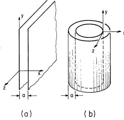
Fig. 13.2.1 (a) Plane parallel perfectly conducting plates. (b) Coaxial geometry in which z -independent fields of (a) might be approximately obtained without edge effects.
