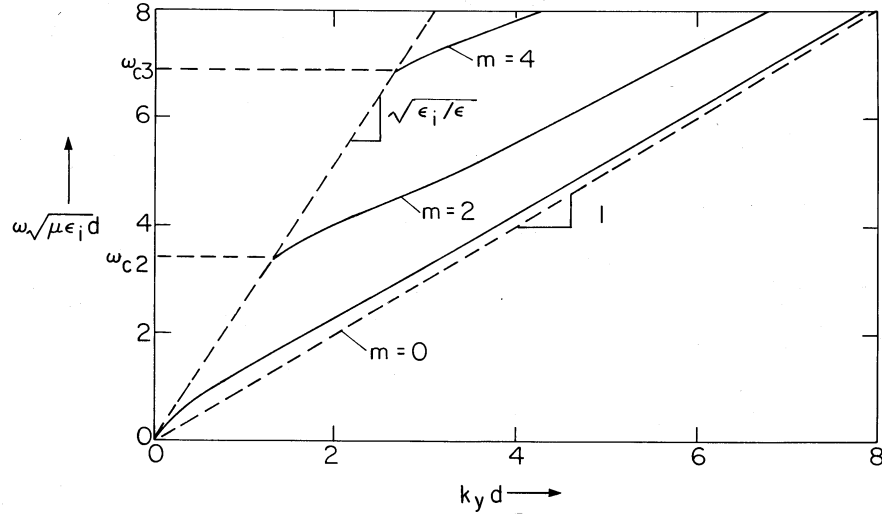
Fig. 13.5.3 Dispersion equation for even TE modes with \epsilon_i/\epsilon = 6.6 .
