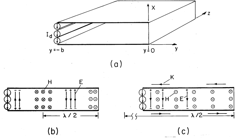
Fig. 13.1.3 (a) Shorted transmission line driven by a distributed current source. (b) Standing wave fields with \mathbf{E} and \mathbf{H} shown at times differing by 90 degrees. (c) MQS fields in limit where wavelength is long compared to length of system.
