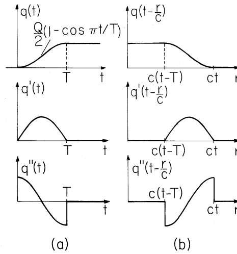
Fig. 12.2.5 (a) Time dependence of the dipole charge q(t) as well as its first and second derivatives. (b) The radial dependence of the functions needed to evaluate the dipole fields resulting from the turn-on transient of (a) when t > T .
