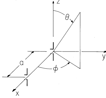
Fig. 12.4.5 Array consisting of two elements with spacing, a .
