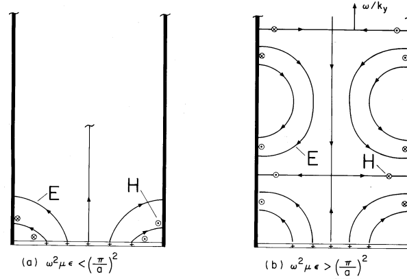
Fig. 12.7.4 The n = 1 TM fields between parallel plates (a) evanescent in y direction and (b) propagating in y direction.
