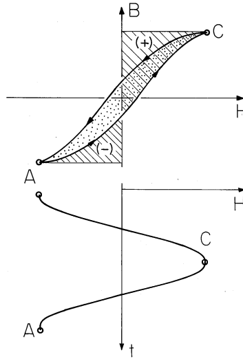
Fig. 11.5.4 With the application of a sinusoidal magnetic field intensity, a steady state is reached in which the hysteresis loop shown in the B-H plane is traced out in the direction shown. The dashed area represents the energy density associated with upward traversal from A to C . The dotted area inside the loop represents the energy density dissipated per traversal of the loop.
