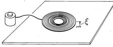
Fig. 11.7.5 When the pancake coil is driven by an ac current, it floats above the aluminum plate. In this experiment, the coil consists of 250 turns of No. 10 copper wire with an outer radius of 16 cm and an inner one of 2.5 cm. The aluminum sheet has a thickness of 1.3 cm. With a 60 Hz current i of about 20 amp rms, the height above the plate is 2 cm.
