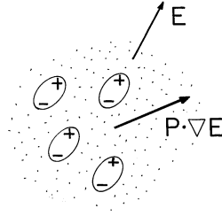
Fig. 11.9.3 The electric Kelvin force density results because the force on the individual dipoles is passed on to the neutral medium.
