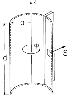
Fig. 11.2.2 One-turn solenoid surrounding volume enclosed by surface S denoted by dashed lines. Poynting flux through this surface accounts for the rate of change of magnetic energy stored in the enclosed volume.
