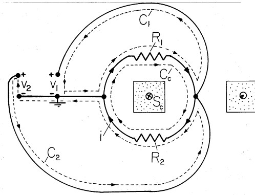
Fig. 10.0.2 Schematic of circuit for experiment of Fig. 10.0.1, showing contours used with Faraday's law to predict the differing voltages v_1 and v_2 .
