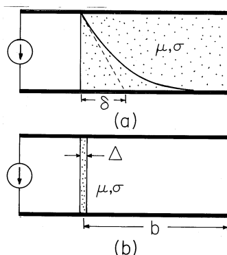
Fig. 10.7.5 Perfectly conducting \mathcal{D} -shaped conductors are driven by a distributed current source at the left. The magnetic field is shielded out of the region to the right enclosed by the perfect conductors by: (a) a block of conductor that fills the region and has a thickness b that is large compared to a skin depth; and (b) a sheet conductor having a thickness \Delta that is less than the skin depth.
