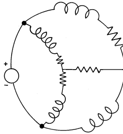
Fig. 10.0.3 Magnetoquasistatic systems with Ohmic conductors are generalizations of inductor-resistor networks. The steady current distribution is determined by the resistors, while the high-frequency response is governed by the inductors.
