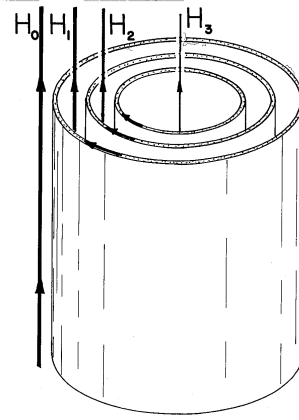
Fig. 10.5.2 Example of an axial field configuration composed of coaxial conducting shells of infinite axial length. When an exterior field H_0 is applied, currents circulating in the shells tend to shield out the imposed field.
