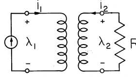
Fig. 9.7.8 Transformer with a load resistance R that includes the internal resistance of the secondary winding.
