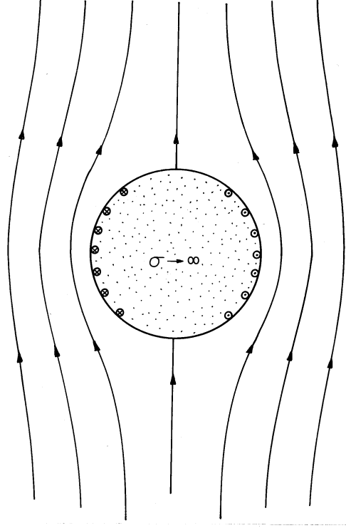
Fig. 8.4.2 Lines of magnetic field intensity for perfectly conducting cylinder in transverse magnetic field.
