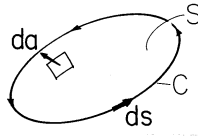
Fig. 8.6.1 Open surface S having area element d\mathbf{a} enclosed by contour C having directed differential length d\mathbf{s} .
