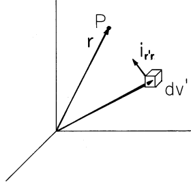
Fig. 8.2.2 Source coordinate \mathbf{r}' and observer coordinate \mathbf{r} showing unit vector \mathbf{i}_{\mathbf{r}'\mathbf{r}} directed from \mathbf{r}' to \mathbf{r} .
