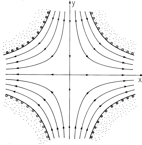
Fig. 8.6.4 Surfaces of constant A_z and hence lines of magnetic field intensity for field trapped between perfectly conducting electrodes.
