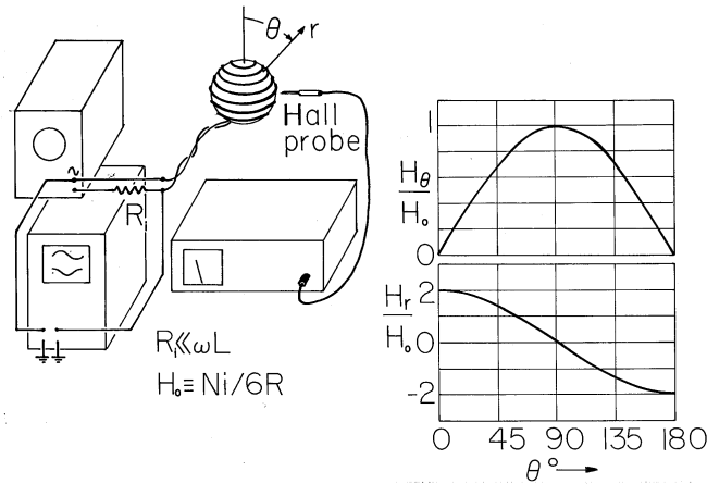
Fig. 8.5.5 Demonstration of fields surrounding the magnetic “flux ball.”
