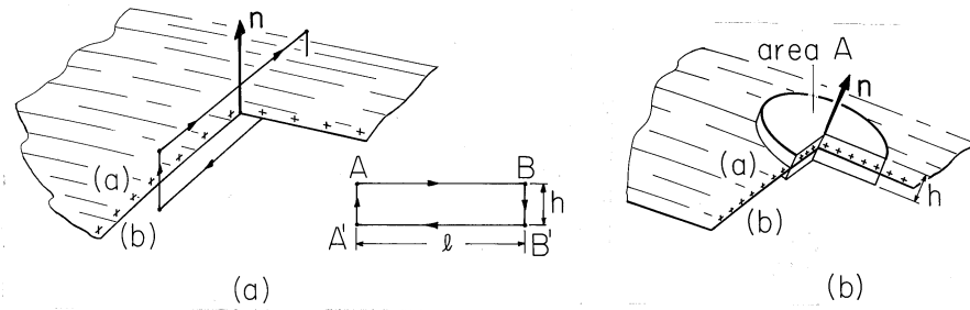
Fig. 5.3.1 (a) Differential contour intersecting surface supporting surface charge density. (b) Differential volume enclosing surface charge on surface having normal \mathbf{n} .
