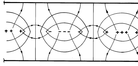
Fig. 5.6.4 Equipotentials and field lines caused by ac part of sheet charge in the configuration of Fig. 5.6.3.
