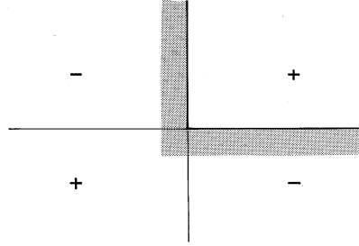
Fig. 4.7.3 Image charges arranged to satisfy equipotential conditions in two planes.
