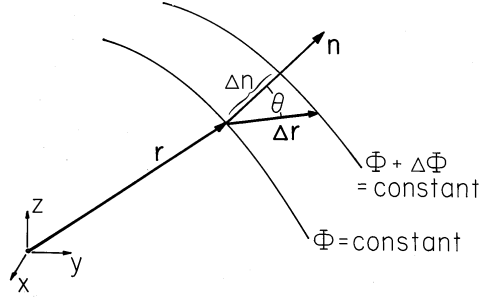
Fig. 4.1.2 Two equipotential surfaces shown cut by a plane containing their normal, \mathbf{n} .
