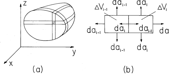
Fig. 2.2.1 (a) Three mutually perpendicular slices define an incremental volume in the volume V shown in cross-section. (b) Adjacent volume elements with common surface.
