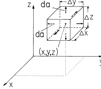
Fig. 2.1.1 Incremental volume element for determination of divergence operator.
