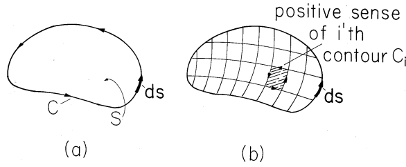
Fig. 2.5.1 Arbitrary surface enclosed by contour C is subdivided into incremental elements, each enclosed by a contour having the same sense as C .
