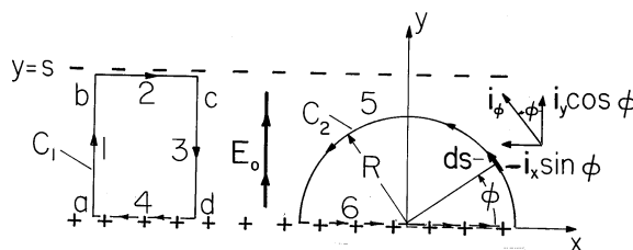
Fig. 1.6.2 Uniform electric field intensity E_o , between plane parallel uniform distributions of surface charge density, has no circulation about contours C_1 and C_2 .
