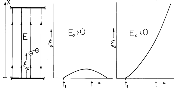
Fig. 1.1.2 An electron, subject to the uniform electric field intensity E_x , has the position \xi_x , shown as a function of time for positive and negative fields.
