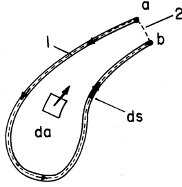
Fig. 1.6.3 Line segment (1) through a perfectly conducting wire and (2) joining the terminals (a) and (b) form closed contour.
