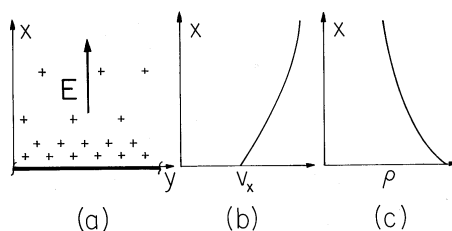
Fig. 1.2.2 Charge injected at the lower boundary is accelerated upward by an electric field. Vertical distributions of (a) field intensity, (b) velocity and (c) charge density.
