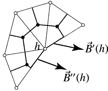
Figure 12: Equilibrium applied to the incomplete dual cell of a boundary node h .
