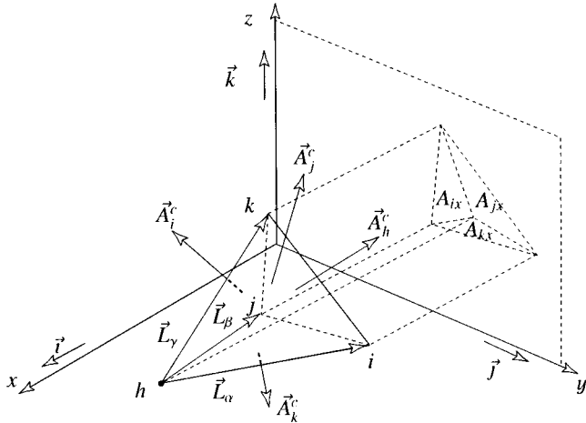
Figure 14: The projections of the tetrahedra faces on the yz plane.
