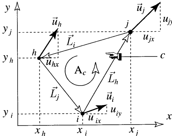
Figure 7: The three nodal displacements relative to the primal cell c .
