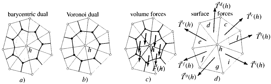
Figure 11: The auxiliary polygon is the same for barycentric and Voronoi dual cells.
